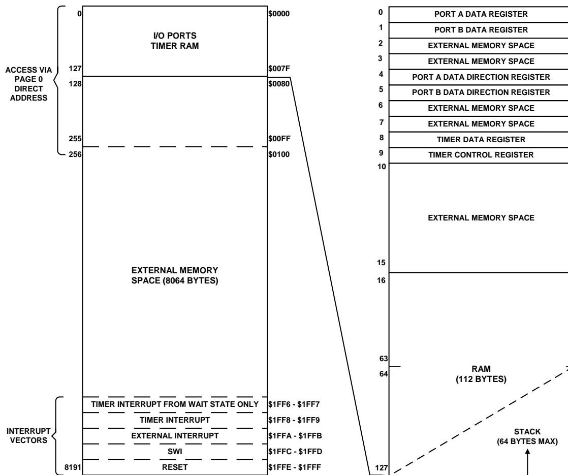
Figure 5. Memory Map
